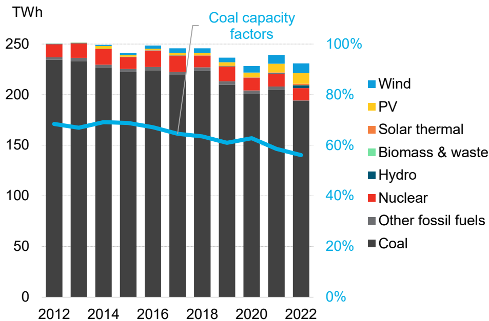
Source: BloombergNEF, Nersa. Note: 'Other fossil fuels' includes oil and diesel. Coal capacity factors are the fleet-wide average and not de-rated for availability.
