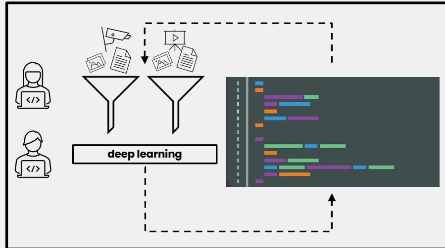
Software 2.0
