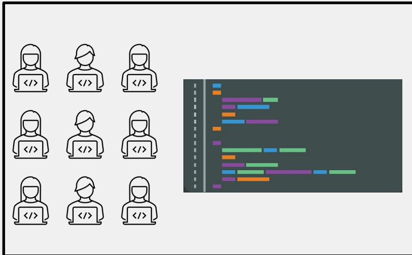
Software 1.0
